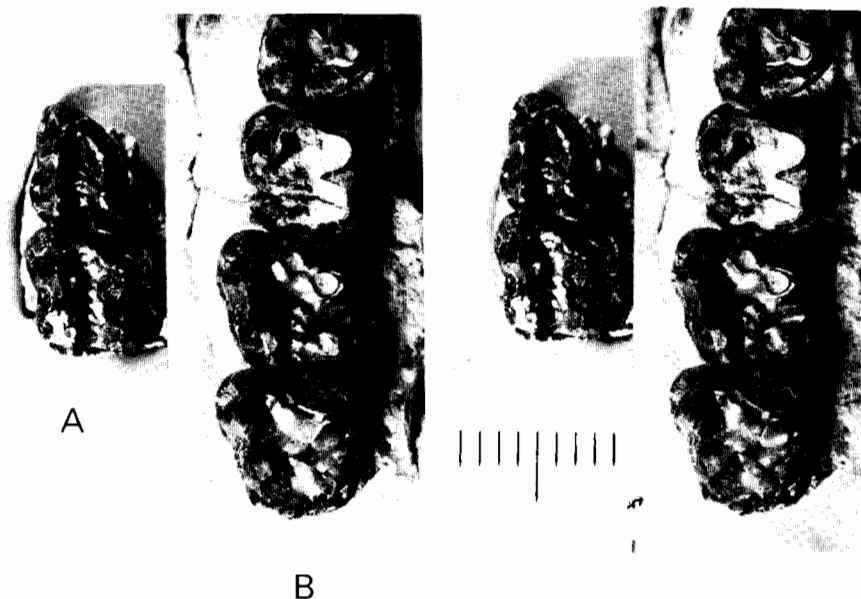
FIG. 23. Hyracotherium angustidens from the Powder River local fauna. A. AMNH 56175, dP_3 - M_4 , Reculosa Blowout. B. AMNH 56174, right P_4 - M_3 , Dry Well locality.
