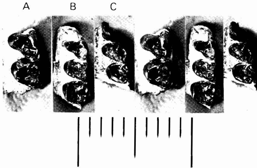
FIG. 22. Apheliscus nitidus from the early Wasatchian. A. AMNH 15849, type, left P^4-M^1 , Gray Bull (?Sand Coulee), Bighorn Basin. B. AMNH 56329, left P^4-M^2 , Dry Well locality, Powder River local fauna. C. AMNH 16935, right P^3-M^1 (photographically reversed), Gray Bull (South Elk Creek), Bighorn Basin, type of " Parapheliscus wapitiensis ."
