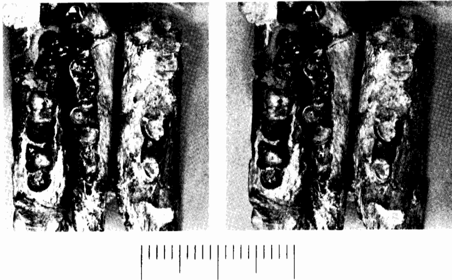
FIG. 10. ? Paeneprolimnocyon mordax . Left, AMNH 16157, type, right M_{1-3} , "middle" Gray Bull, Bighorn Basin; center, AMNH 56320, left M_{1-3} , Bozeman locality, Powder River local fauna; right, AMNH 15168, (type Prolimnocyon robustus ), right M_{2-3} , "middle" Gray Bull, Bighorn Basin.
