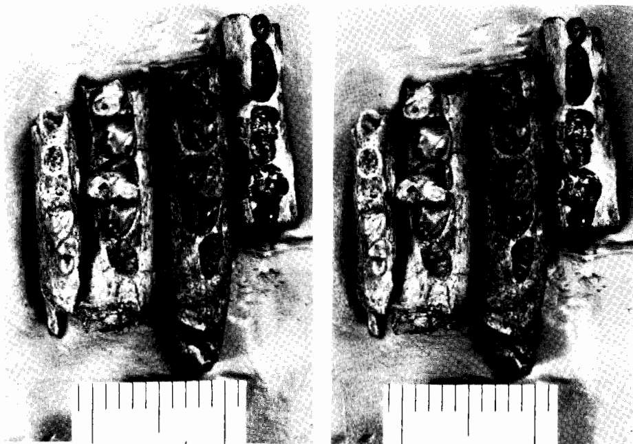
FIG. 12. Prolimnocyon atavus . Left to right: AMNH 56319, left M_{2-3} , Reculusa Blowout, Powder River local fauna; AMNH 16816, type, left M_{1-3} , late Gray Bull, Bighorn Basin; AMNH 16817, left M_{1-3} , "middle" Gray Bull, Bighorn Basin; AMNH 56216, right P_4-M_2 , Bozeman locality, Powder River local fauna.
